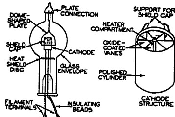
Mercury-vapor rectifier—typical construction.
